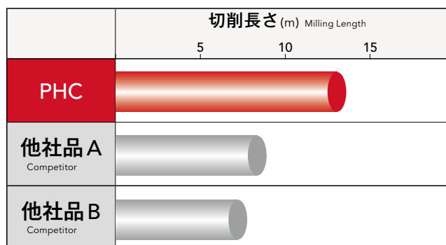
PHC (13.2m加工時点) After 13.2m of milling
